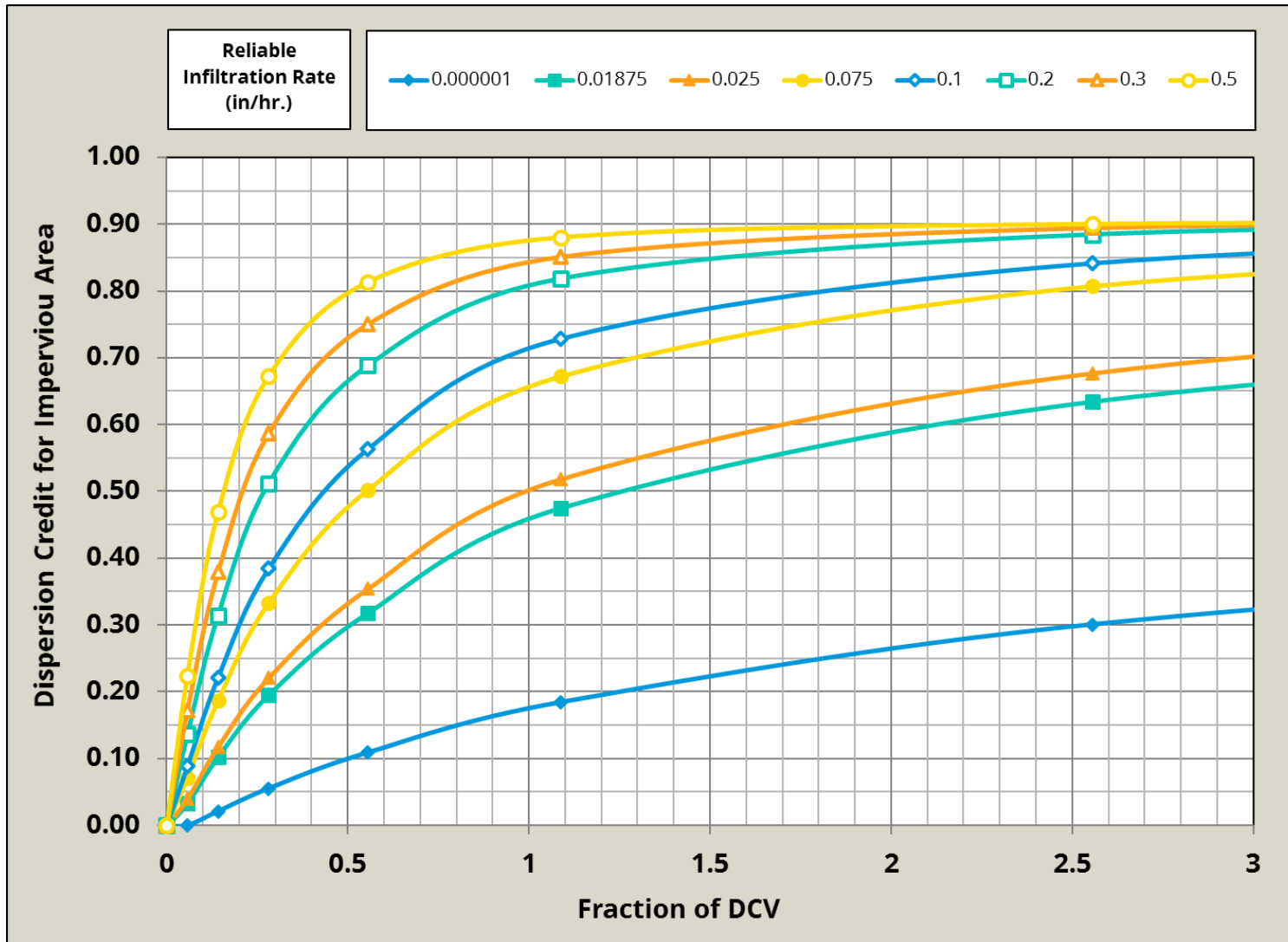
Figure B.5-8. 9 th Amendment Dispersion Nomographs
