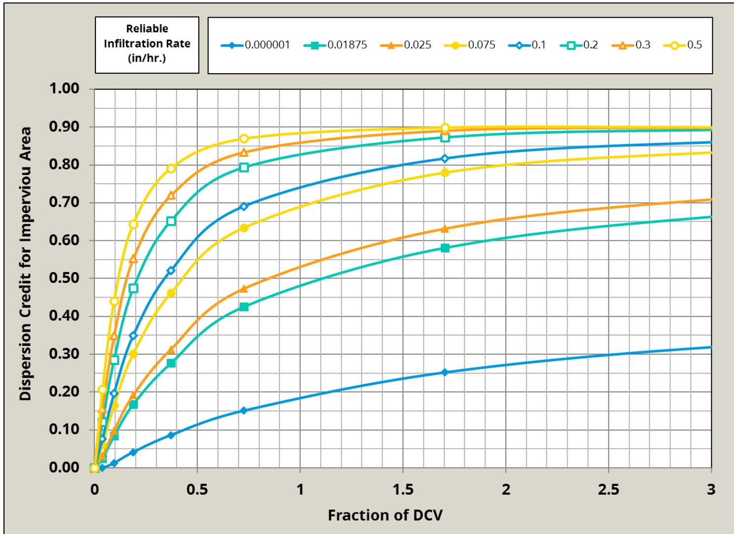
Figure B.5-7. 6” Amendment Dispersion Nomographs
