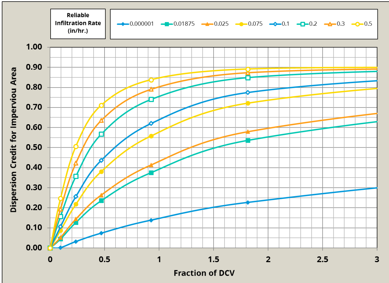
Figure B.5-10. 15" Amendment Dispersion Nomographs
