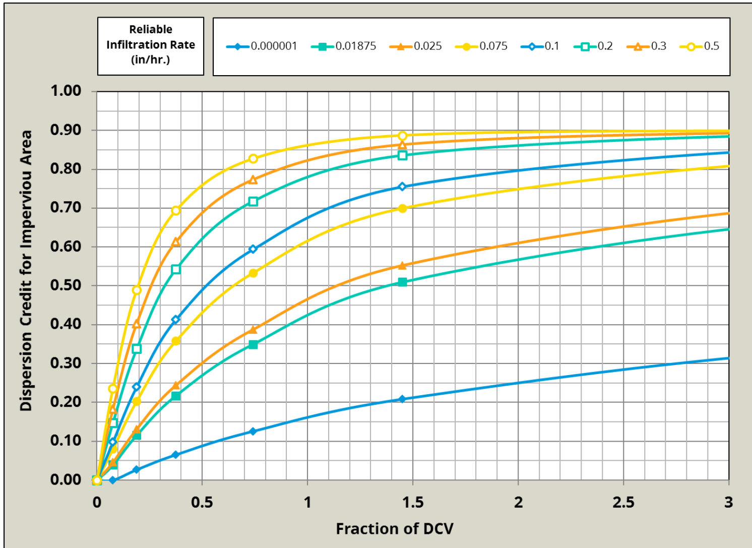
Figure B.5-9. 12" Amendment Dispersion Nomographs
