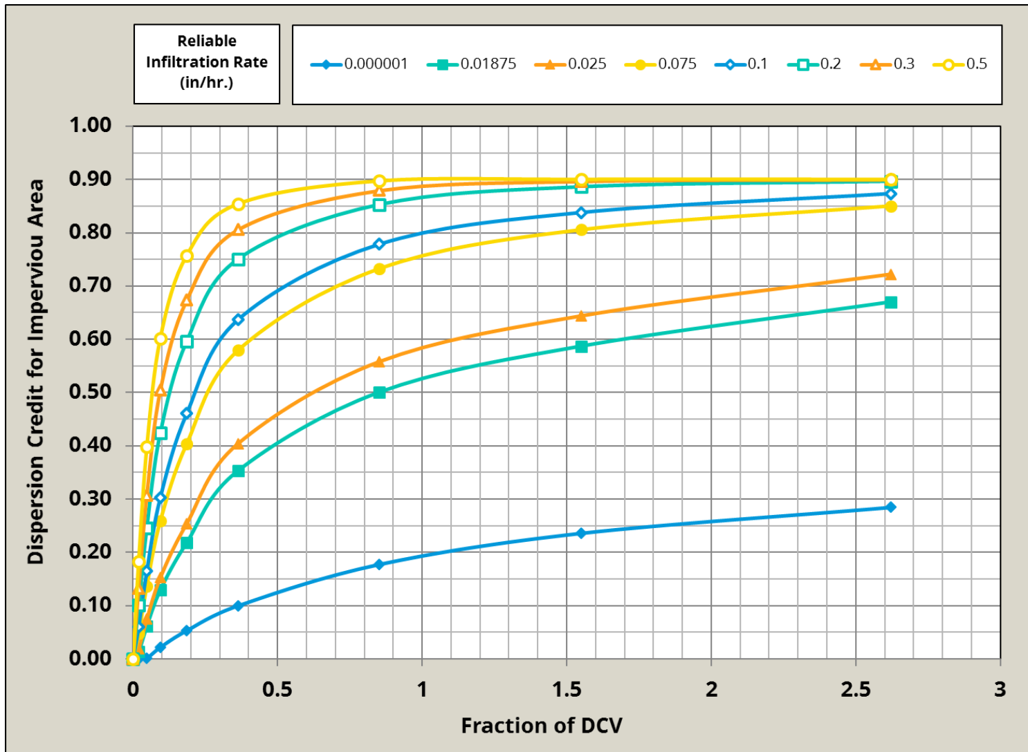
Figure B.5-6. 3” Amendment Dispersion Nomographs
