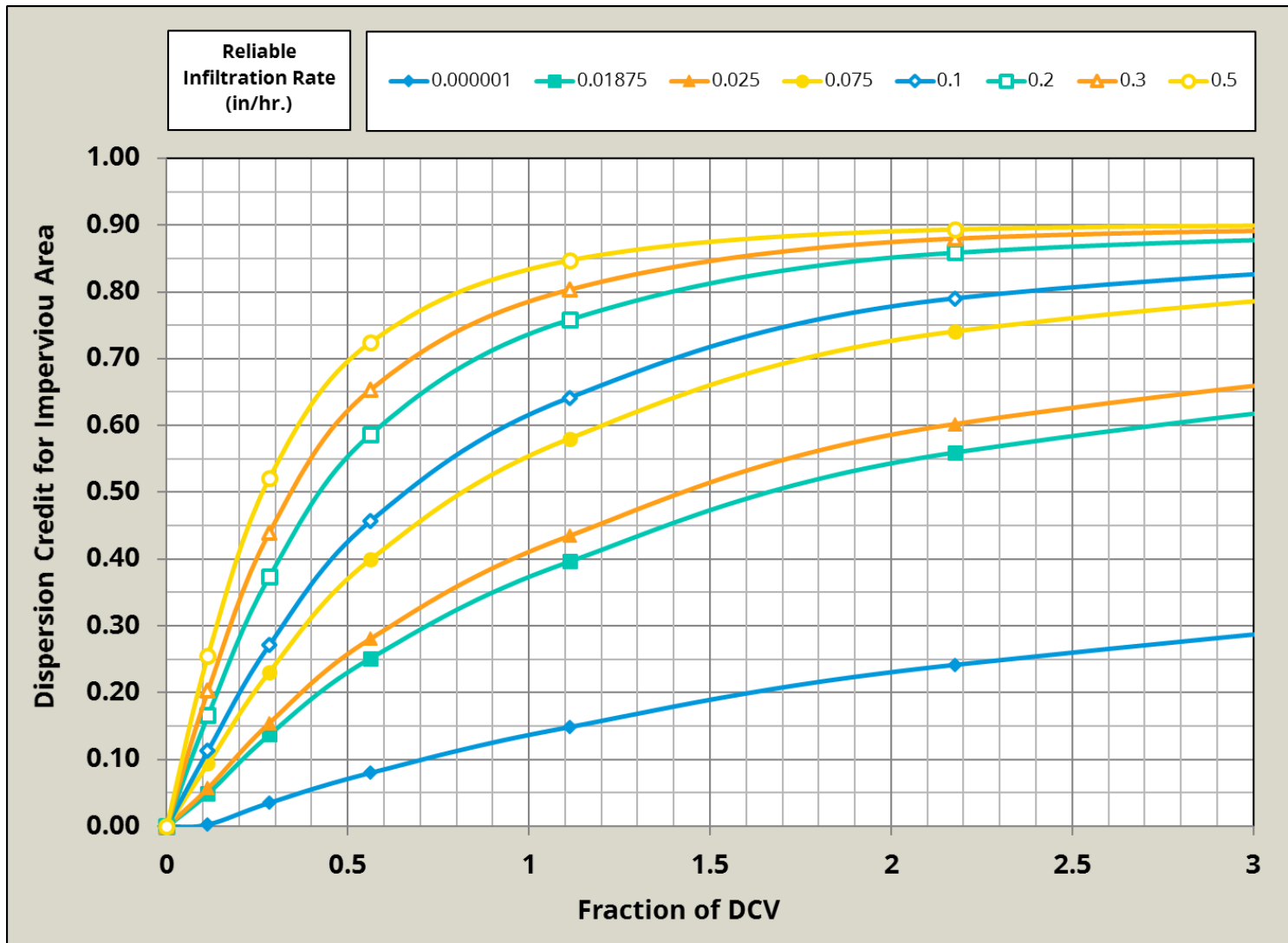
Figure B.5-11. 18” Amendment Dispersion Nomographs
