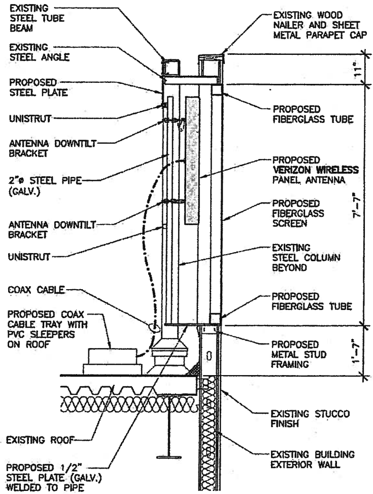
ANTENNA SECTION
