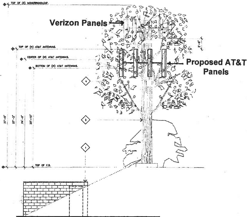
NORTH ELEVATION
