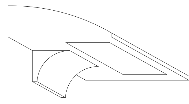
TYPICAL WALL PACK DETAIL SCALE: NTS
