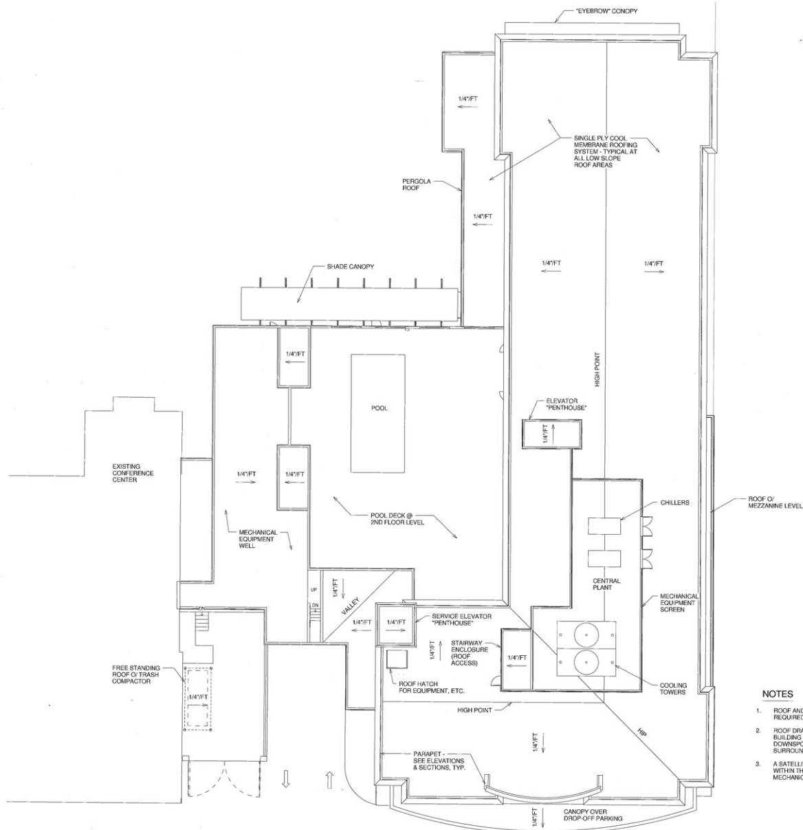
1 Roof Plan 3/32" = 1'-0"
