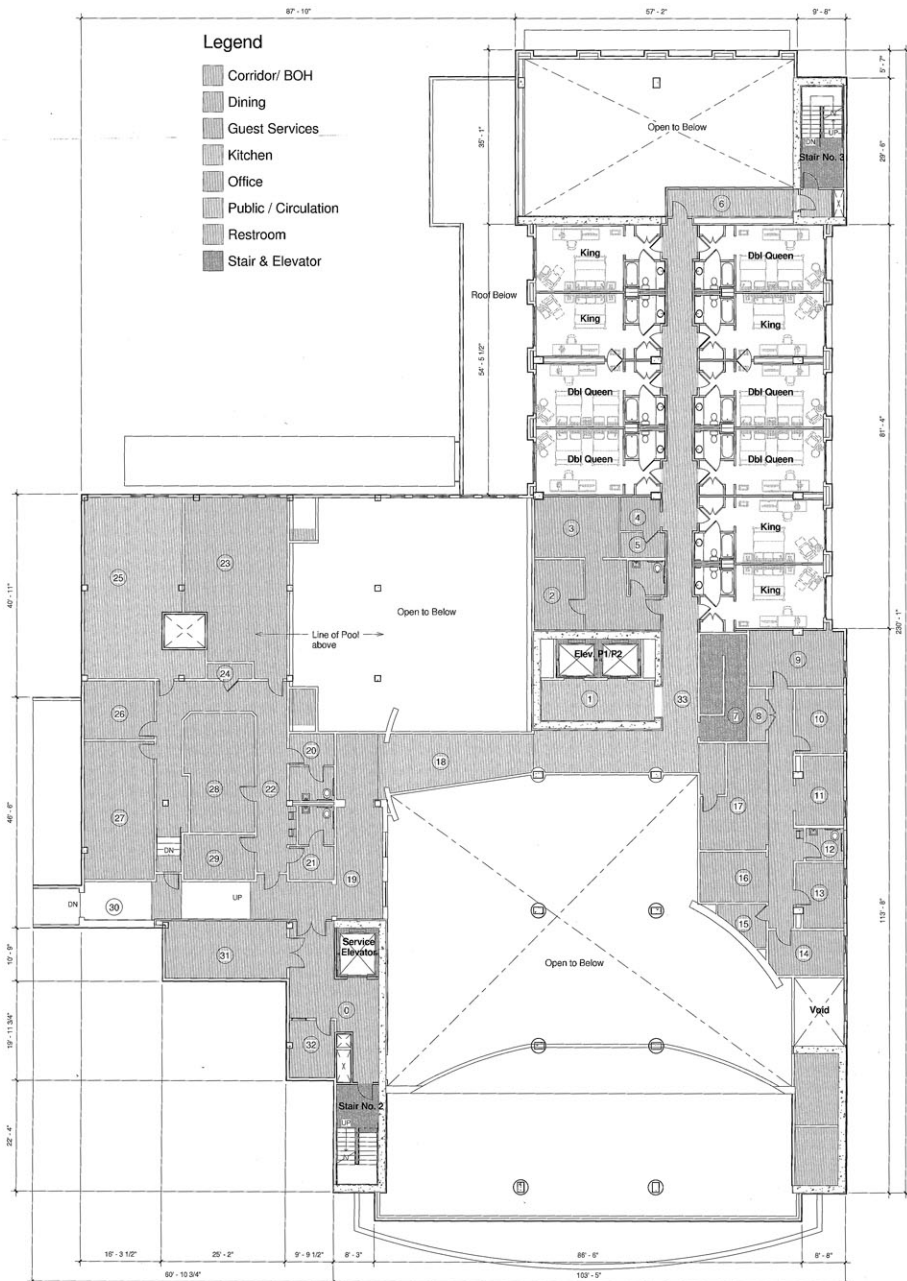
1 Mezzanine Floor Plan 3/32" = 1'-0"
