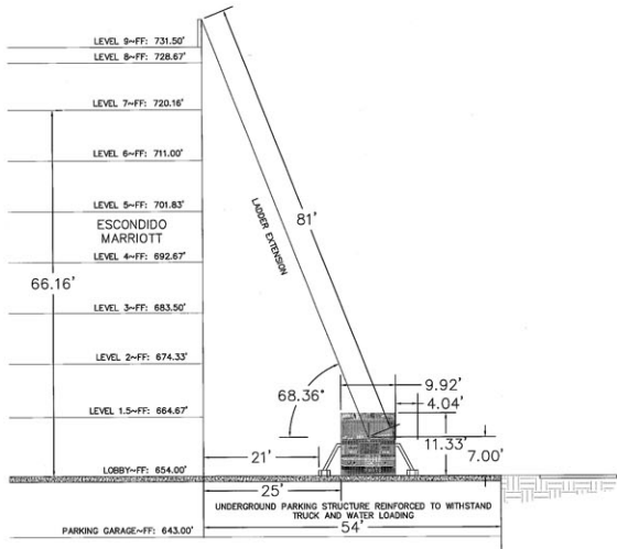
NORTH SECTION 1"=10'
