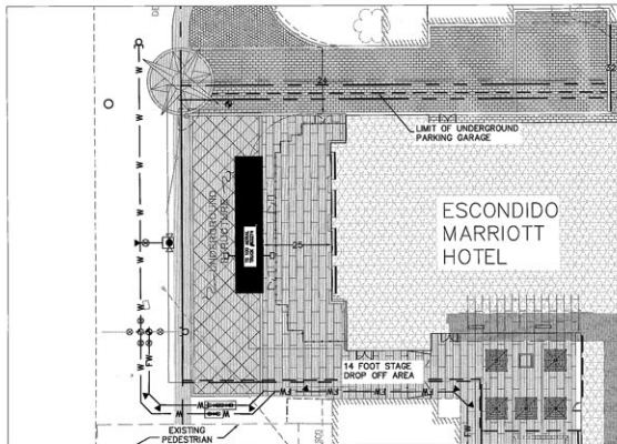
NORTH PLAN 1"=20'
