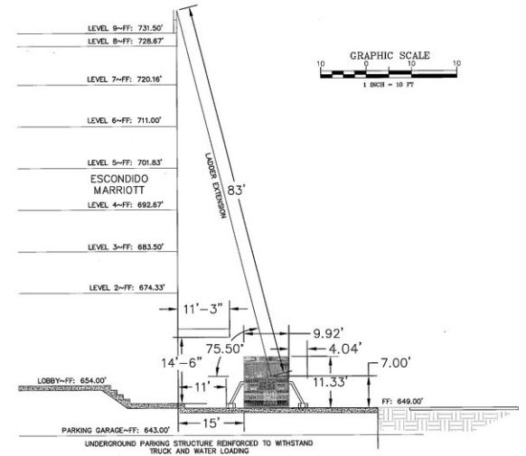
SOUTH SECTION - 1"=10'
