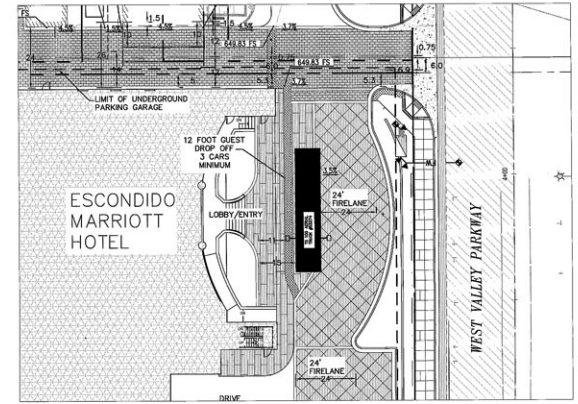
SOUTH PLAN - 1"=20'
