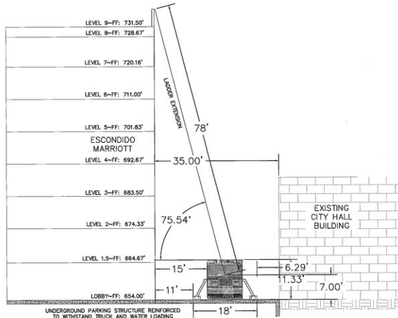
EAST SECTION - 1"=10'
