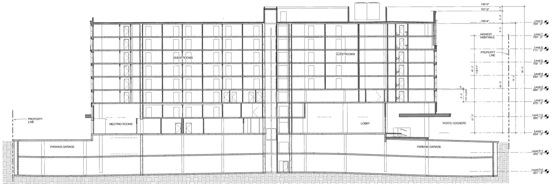
1 Longitudinal Section 'A' 3/32" = 1'-0"
