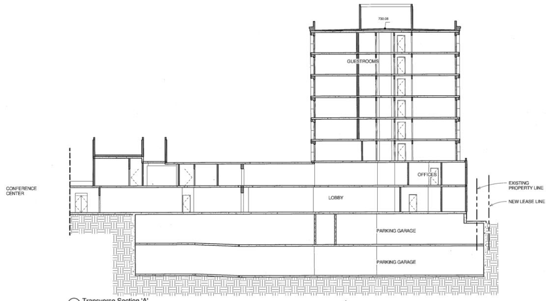
2 Transverse Section 'A' 3/32" = 1'-0"
