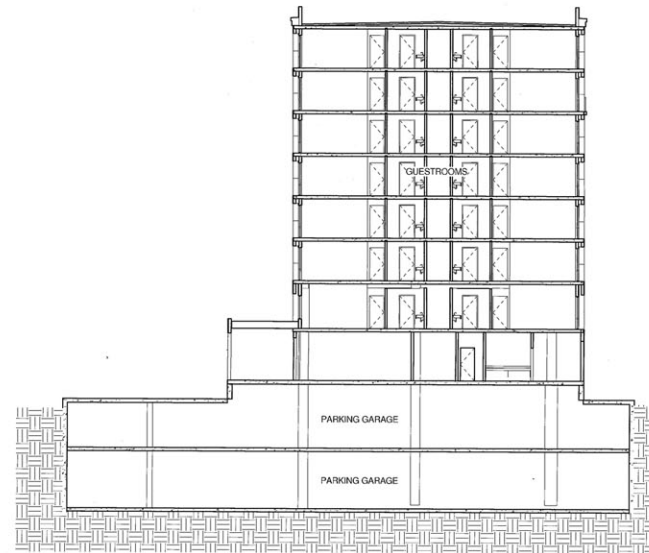
2 Transverse Section 'B' 3/32" = 1'-0"
